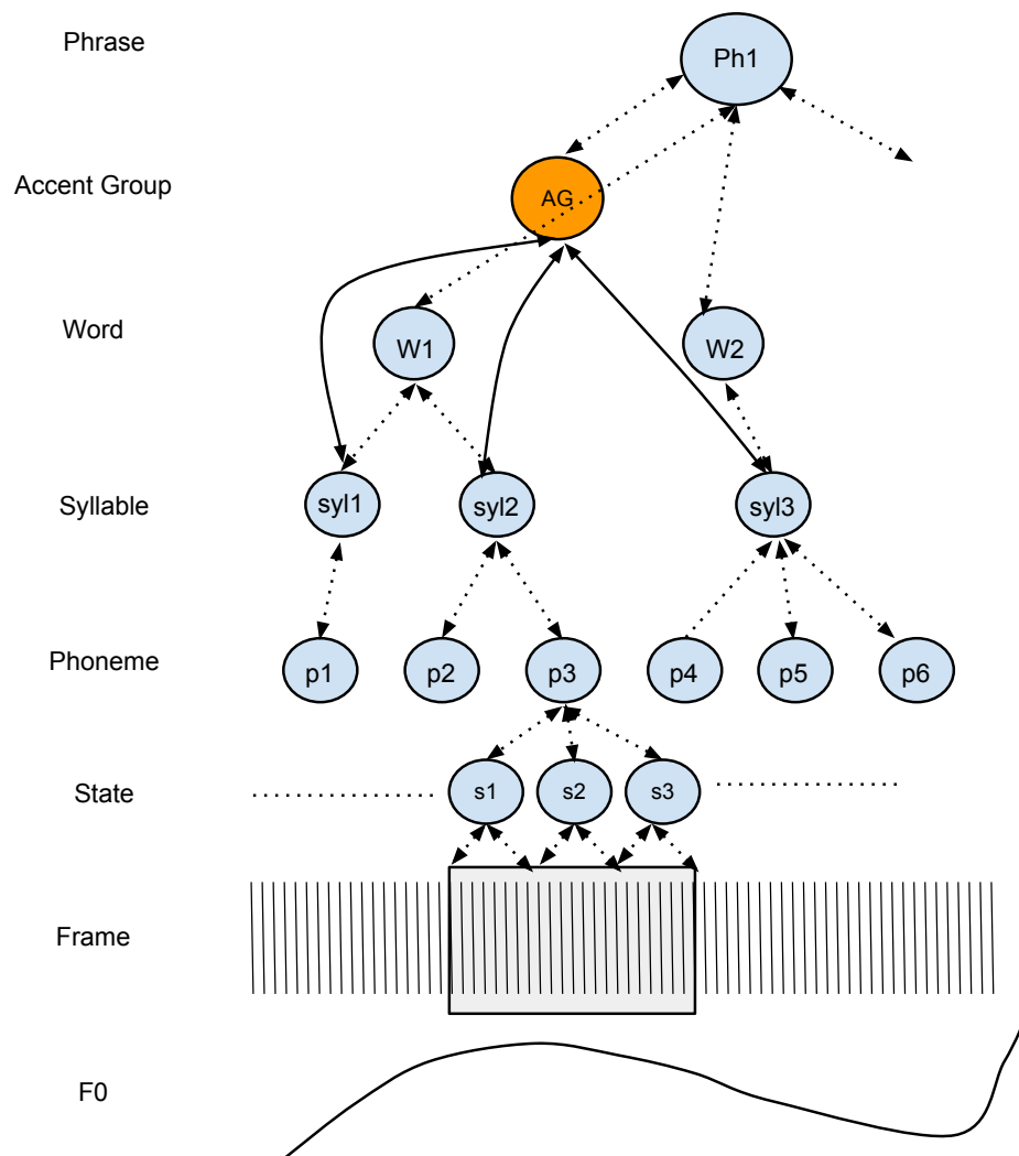
Figure 3.6: Illustration of the proposed prosodic structure in Festival. The new Accent Group relation is highlighted.
