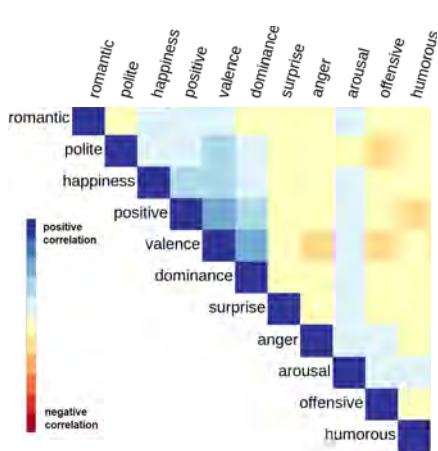
Figure 1.8: Cross-stylization.
