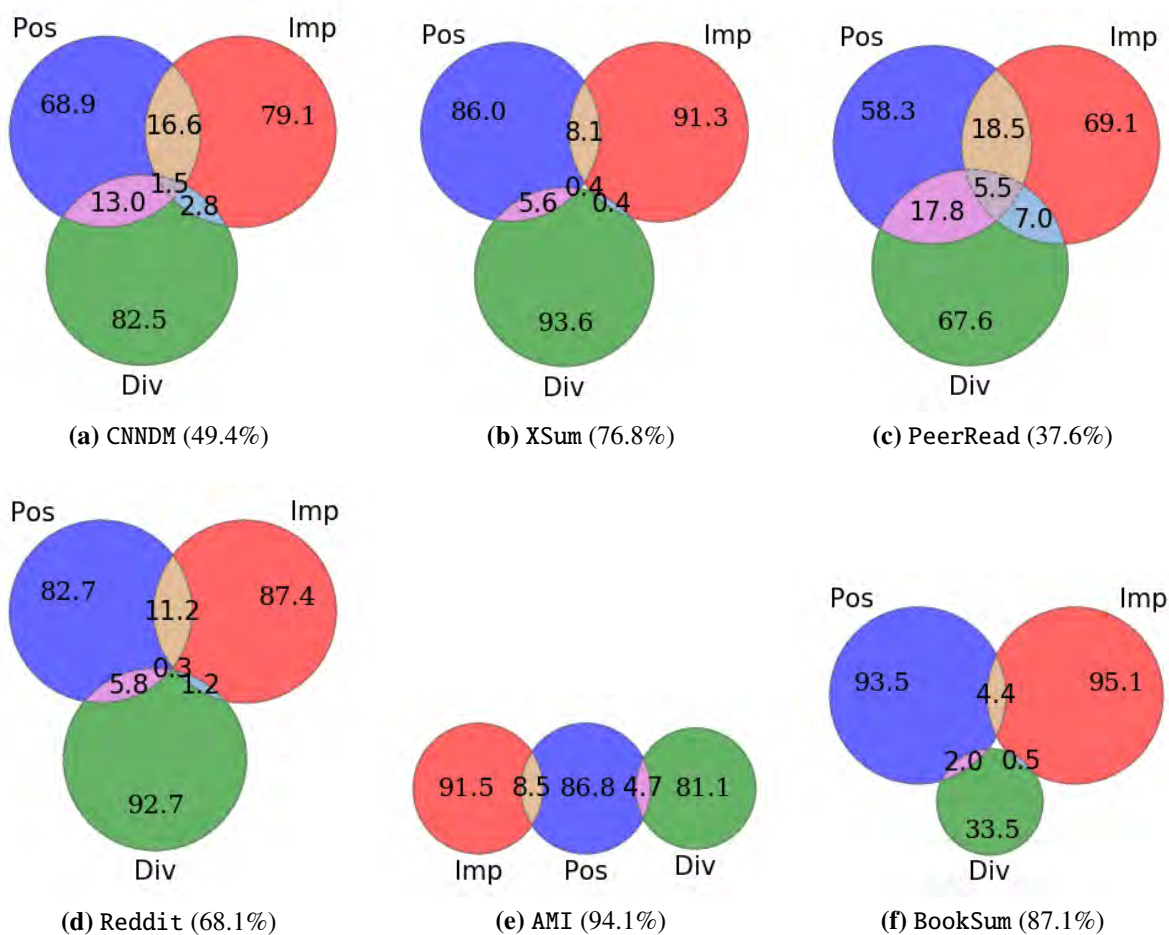
Figure 3.22: Intersection of averaged summary sentence overlaps across the sub-aspects. We use First for POSITION, ConvexFall for DIVERSITY, and N-Nearest for IMPORTANCE. The number in the parenthesis called Oracle Recall is the averaged ratio of how many the oracle sentences are NOT chosen by union set of the three sub-aspect algorithms. Other corpora are in Appendix with their Oracle Recalls: Newsroom(54.4%), PubMed (64.0%) and MScript (99.1%).
