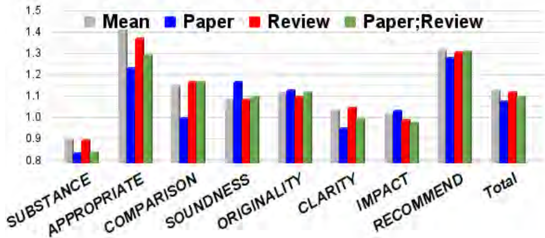
Figure 3.19: Root mean squared error (RMSE, lower is better) on the test set for the aspect prediction task on the ACL 2017 (top) and the ICLR 2017 (bottom) sections of PeerRead.
