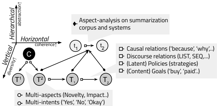
Figure 1.7: Text planning.
