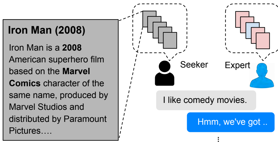
Figure 3.13: Recommendation as a dialogue game. We collect 81,260 recommendation utterances between pairs of human players (experts and seekers) with a collaborative goal: the expert must recommend the correct (blue) movie, avoiding incorrect (red) ones, and the seeker must accept it. A chatbot is then trained to play the expert in the game.
