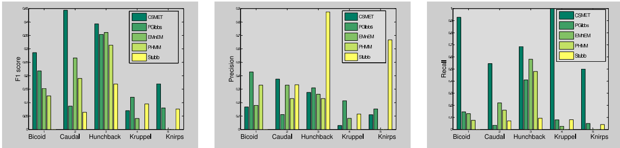
Figure 3.7: Comparison of algorithms on motif search performance over 5 motifs on real CRMs.
