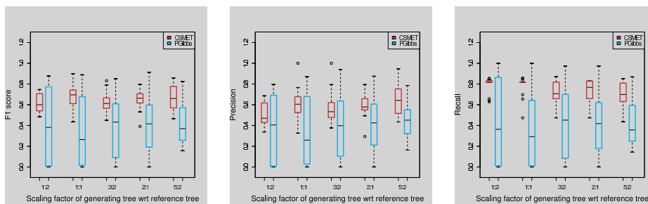
Figure 3.6: Performance on modified PSPE data. The label on the X-axis denotes the scaling factor used by the PSPE tree with respect to a reference Drosophila phylogeny. From [148].
