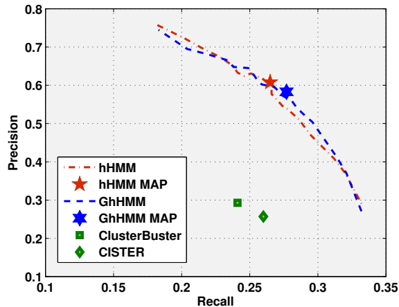
Figure 2.2: The precision-recall curves of two models of BayCis (hHMM and GhHMM) versus the P/R of default predictions by CISTER and ClusterBuster. From [106].
