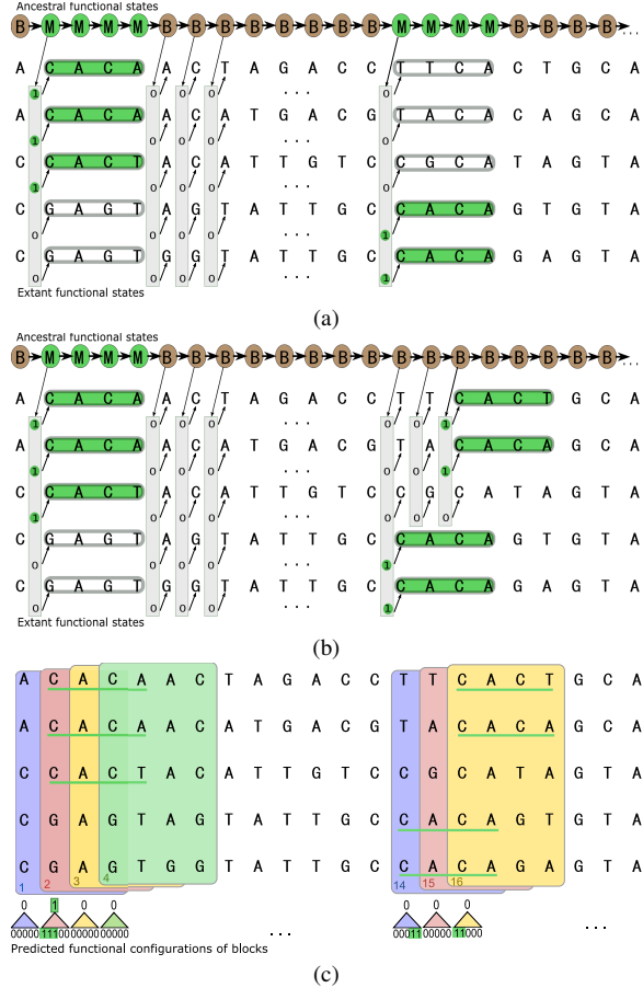
Figure 3.2: Context-specific relationships among variables due to two possible value configurations of hidden variables shown in (a) and (b). Note that when the ancestral state is a motif, the segment corresponding to the TBFS evolves as a unit (as shown by the arrow from an extant functional state pointing to a multi-column segment), either retaining its functionality as a motif, or turning-over to a background segment, as illustrated in (a). When the ancestral state is a background, then every position can evolve independently as long as it is still in the background (as shown by the arrow from a functional state pointing to a single column). But when a motif emerges out of the background, as shown in (b), the segments corresponding to the TFBS start to evolve as a unit, causing even the aligned nucleotide positions to evolve under different positional constraints. Panel (c) outlines the idea of a block approximation of the CSMET emission probability. From [148].
